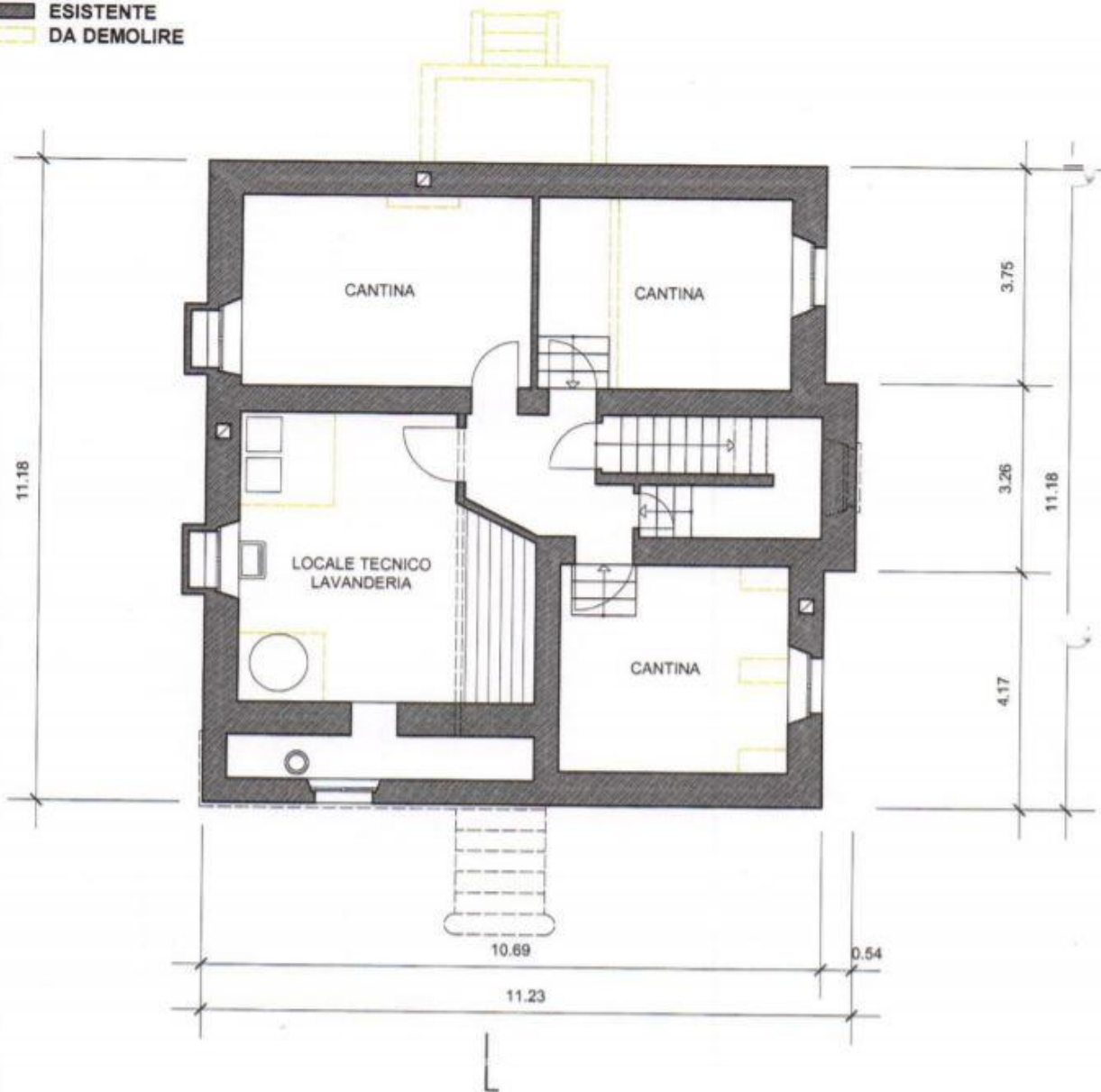
PIANO CANTINATO
